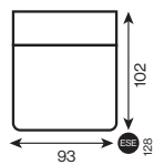
1-seater with electric seat extension
